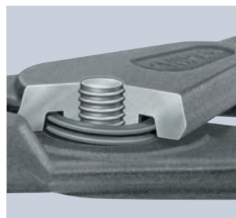
Spring inside the joint: the spring is protected inside the precisely bolted joint. It does not hinder work and cannot get dirty or lost.
