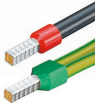
Square compression
