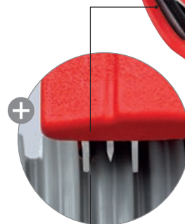
Internal blades with lateral guide to protect against injuries
