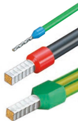
Hexagonal compression
